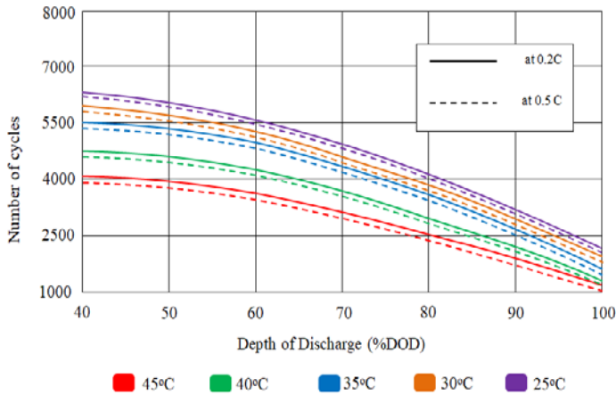
Cycle life versus depth of discharge and temperature
