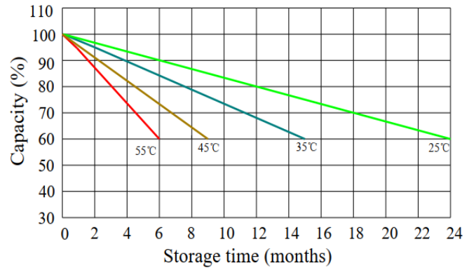
Self-discharge at different temperature
